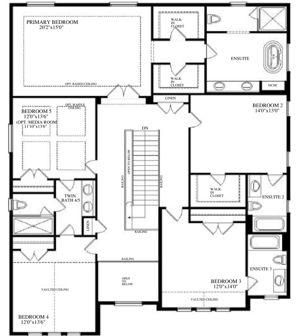
OPT. UPPER LEVEL ELEV. A
